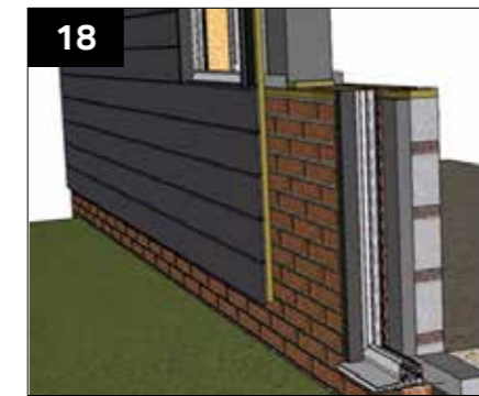
In the case where the new wall is within 1 metre of a boundary Calcium Silicate Board will be provided. This needs to be installed before battening if a cladding is being used.
