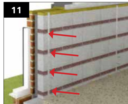
Fixed with a minimum of four hardened nails 4mm in diameter *75mm long, or No12 wood screws *50mm long into plugs (where fixed to masonry). Min 4 fixings required and with the lowest fixing secured within 150mm of the bottom of the vertical strap.
