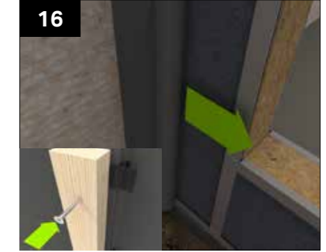
Please follow the steps within the main hup installation guide for installing the membrane and battens with the relevant roof ordered for batten positioning. Ensure the membrane overlaps onto the existing brick by min of 100mm.
