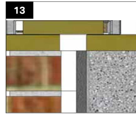
The external wall leaf also has a wallplate added, bedded on mortar to sit level with the internal wallplate. Please ensure these are level with each other.
