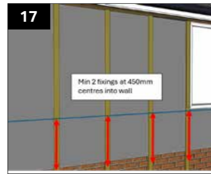
The 25*50mm treated batten running down the outer surface of the wall will be fixed to the wall at a maximum of 450mm centres using No12 screws 75mm long plugged into the wall. Now you can start to install your preferred external finish.
