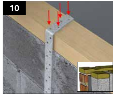
Fix through the top of the wallplate with a minimum of 2 hardened nails 4mm in diameter x 40mm, or min 2 x 4.2 x 38mm woodscrews through the top of the wall strap into the wallplate.
